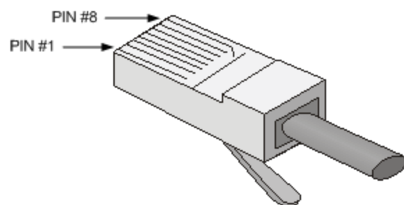
Figure 1 RJ-45 connector
