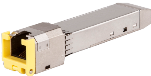
Figure 1 10G SFP+ copper transceiver module
